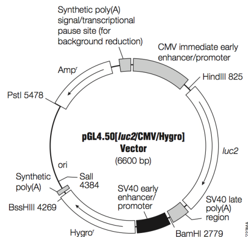
Figure 10 : Plasmide pGL4.50[luc/CMV/Hygro].
